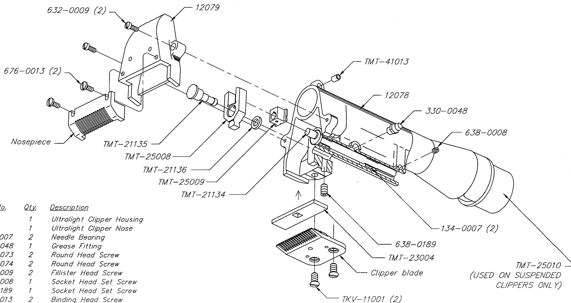
Figure 6 - 12077 Ultralight clipper assembly
